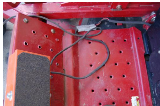
Improper mounting Wires not tied down
